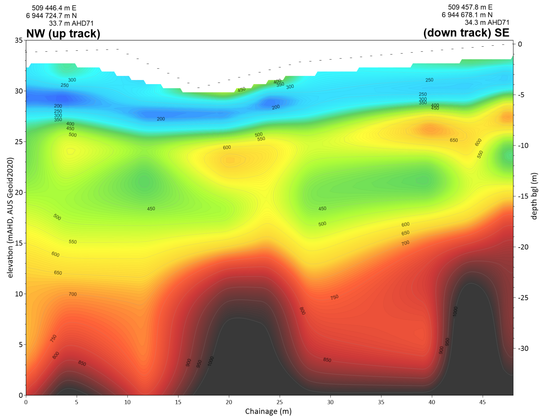
Seismic Line MASW AU-GP 112
